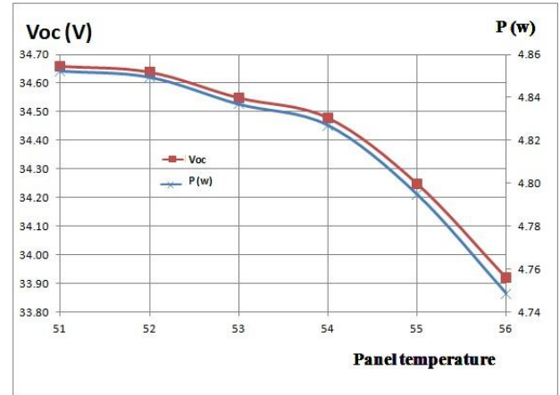
Fig. 3: Effect of panel temperature on Voc
